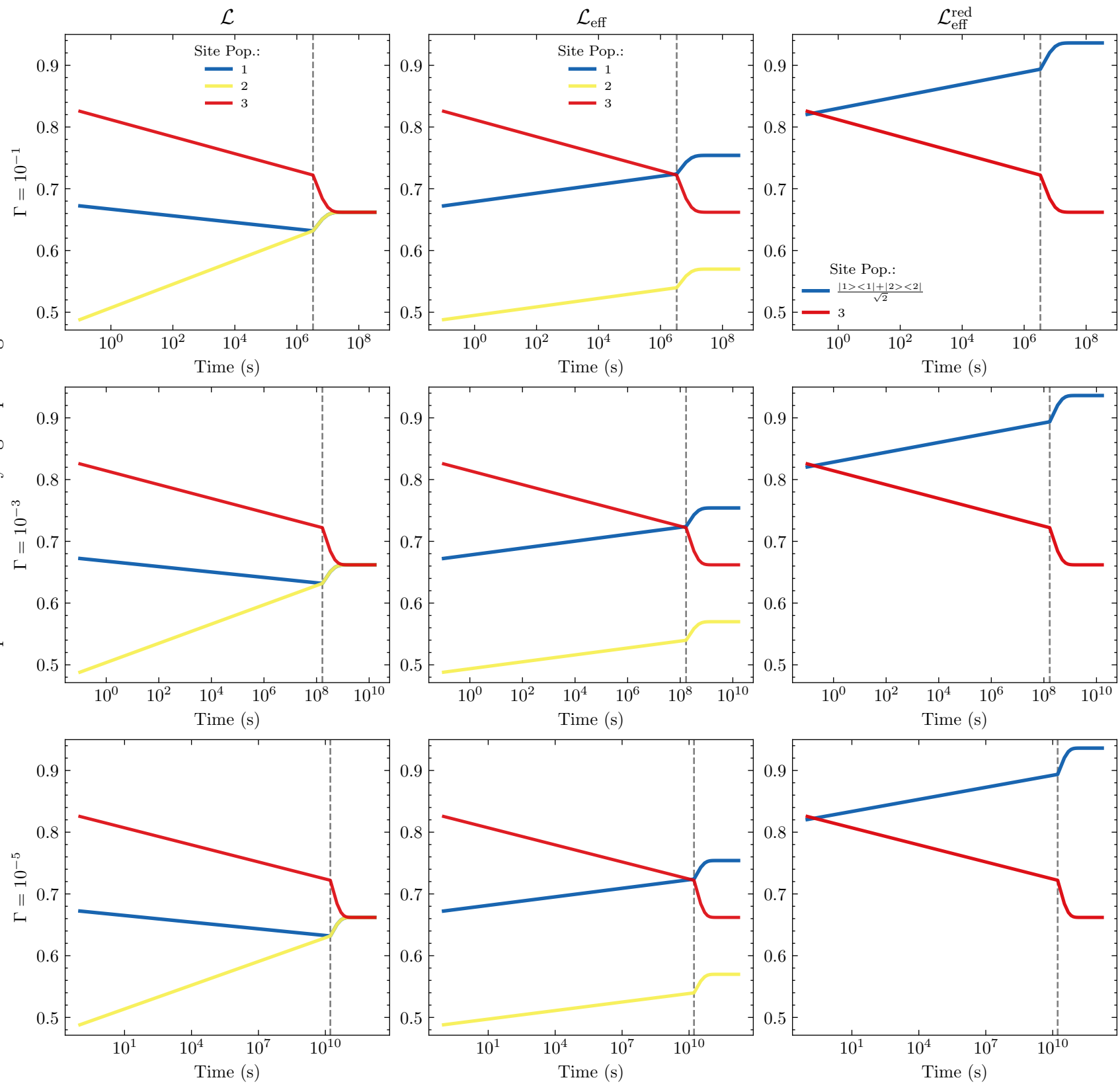
Time Evolution of Site Populations under \mathcal{L} , \mathcal{L}_{\text{eff}} , and \mathcal{L}_{\text{eff}}^{\text{red}}
